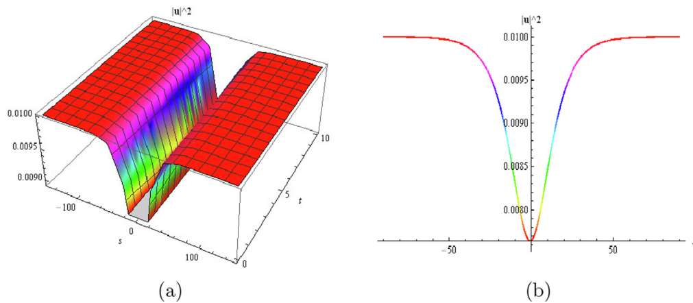
Fig. 3 The (a) 3D surface and (b) 2D surface of Eq. (4.6) under the values, \rho = 0.1 , w = -0.3 , B_0 = 3 , c_1 = 0.3 , B_1 = 0.4 , d_1 = 0.2 and t = 0.123 , for 2D graph.
