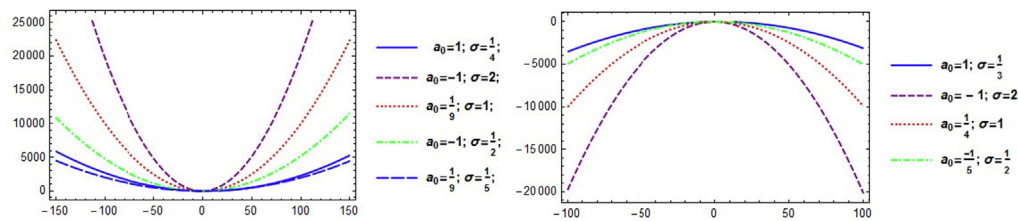
Fig. 9 The modulation instability graphs for different values in Eqs. (5.11) and (5.12).
