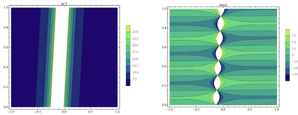
Fig. 2 The contour surfaces of Eq. (4.5) under the values \kappa = 0.1 , \beta = -3 , A_1 = 0.5 , c_1 = 0.3 , B_1 = .0.1 , d_1 = 0.2 .
