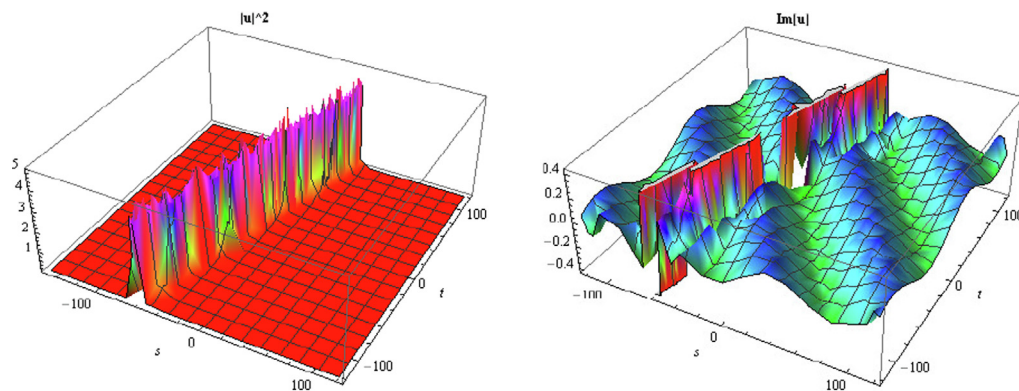
Fig. 7 The 3D surfaces of Eq. (4.11) under the values \lambda = 0.8 , \mu = -0.1 , E = 0.5 , \kappa = 0.3 , \rho = 0.1 , \beta = 0.2 .
