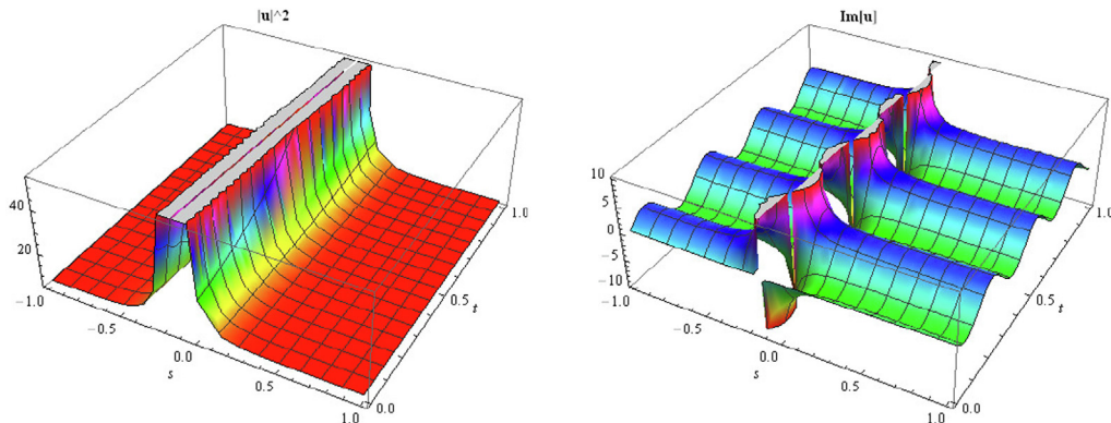
Fig. 1 The 3D surfaces of Eq. (4.5) under the values, \kappa = 0.1, \beta = -3, A_1 = 0.5, c_1 = 0.3, B_1 = .0.1, d_1 = 0.2 .
