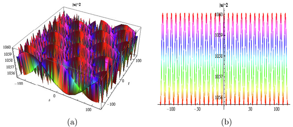
Fig. 8 The (a) 3D surface (b) 2D surface of Eq. (4.14) under the values \lambda = 2 , \mu = 0.2 , E = 0.5 , \kappa = 0.3 , w = 0.1 , B_0 = 0.11 and t = 0.13 for 2D graph.
