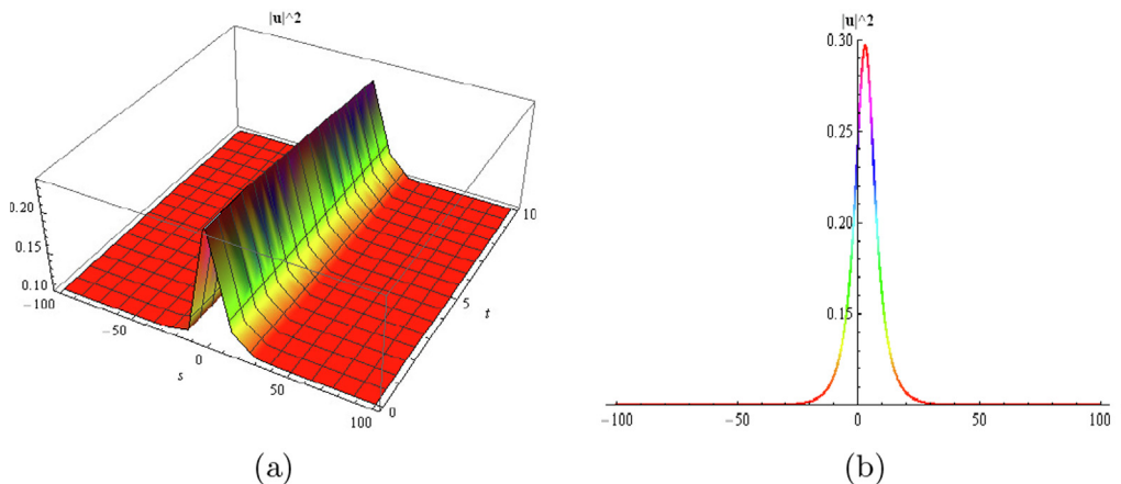
Fig. 4 The (a) 3D surface and (b) 2D surface of Eq. (4.8) under the values, \kappa = 0.1 , \beta = -0.1 , \rho = 0.2 , B_1 = 0.4 , d_1 = 0.5 , c_1 = 0.3 , and t = 0.12 for 2D graph.
