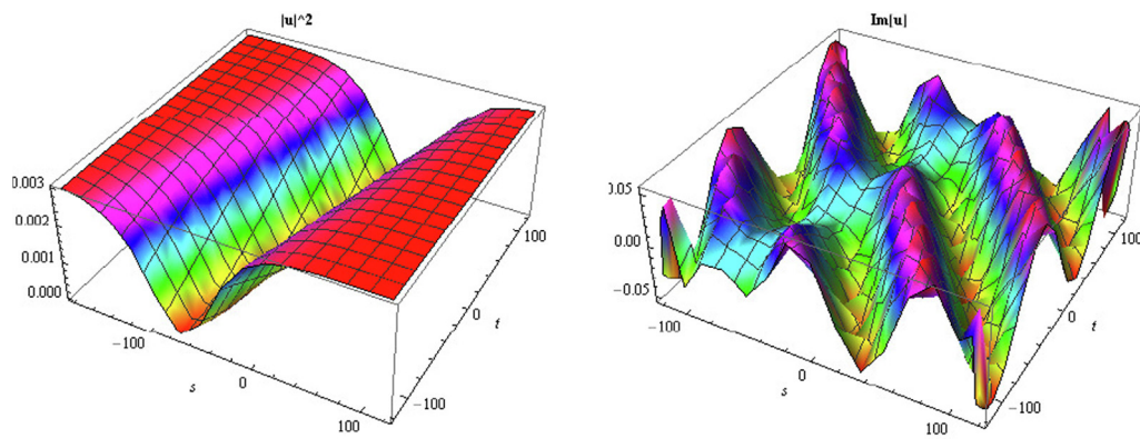
Fig. 5 The 3D surfaces of Eq. (4.10) under the values, \lambda = 0.8 , \mu = 0.1 , E = 0.5 , \kappa = 0.3 , \rho = 0.1 , \beta = 0.2 .
