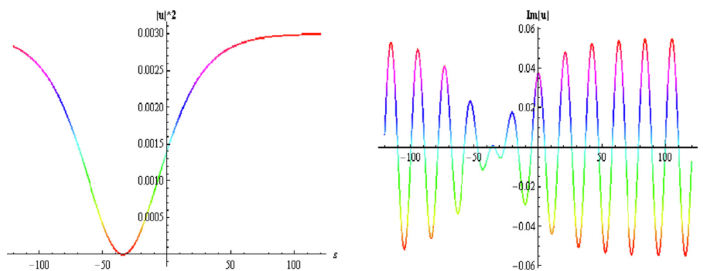
Fig. 6 The 2D surfaces of Eq. (4.10) under the values, \lambda = 0.8 , \mu = 0.1 , E = 0.5 , \kappa = 0.3 , \rho = 0.1 , \beta = 0.2 , t = 0.11 .
