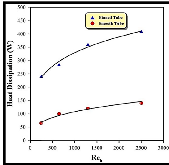
Fig. 6. Influence of the Reynolds number of hot water on heat dispersion at \dot{m}_c = 0.045 kg/s.
