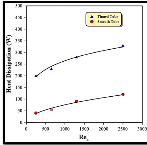
Fig. 5. Influence of the Reynolds number of hot water on heat dispersion at \dot{m}_c = 0.025 kg/s.
