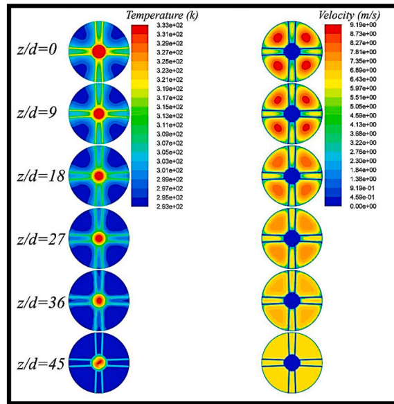
Fig. 16. “Temperature and velocity contours” at Re_h = 1300 , \dot{m}_c = 0.045 kg/sec, and various axial distances for finned tube heat exchanger.
