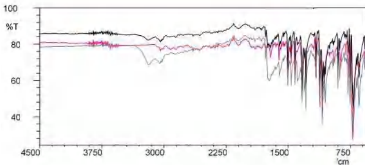
Figure 3. FTIR spectrums of PB15 (pink), D1 (black) and D2 (gray) pigments
