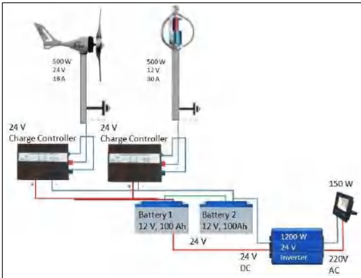
Figure 2. Schematic drawing of the wind energy system
