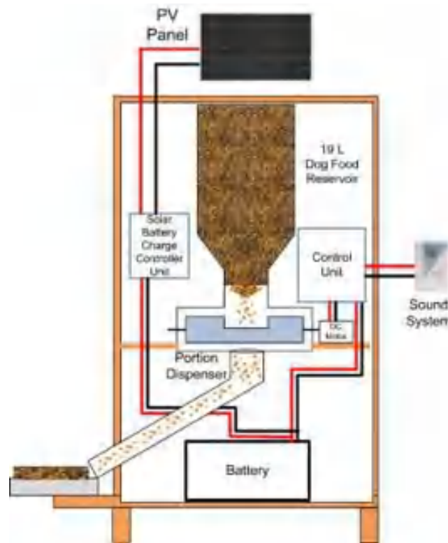
Figure 5. Off-grid solar-powered operation scheme of the automatic pet feeder
