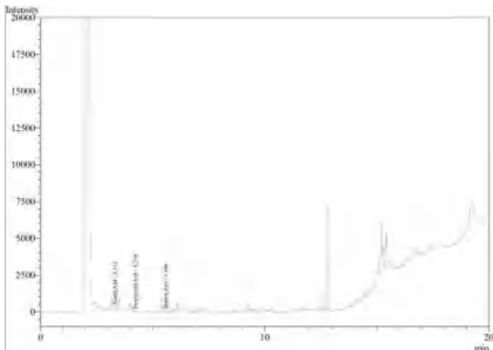
Figure 1. GC-MS chromatogram
