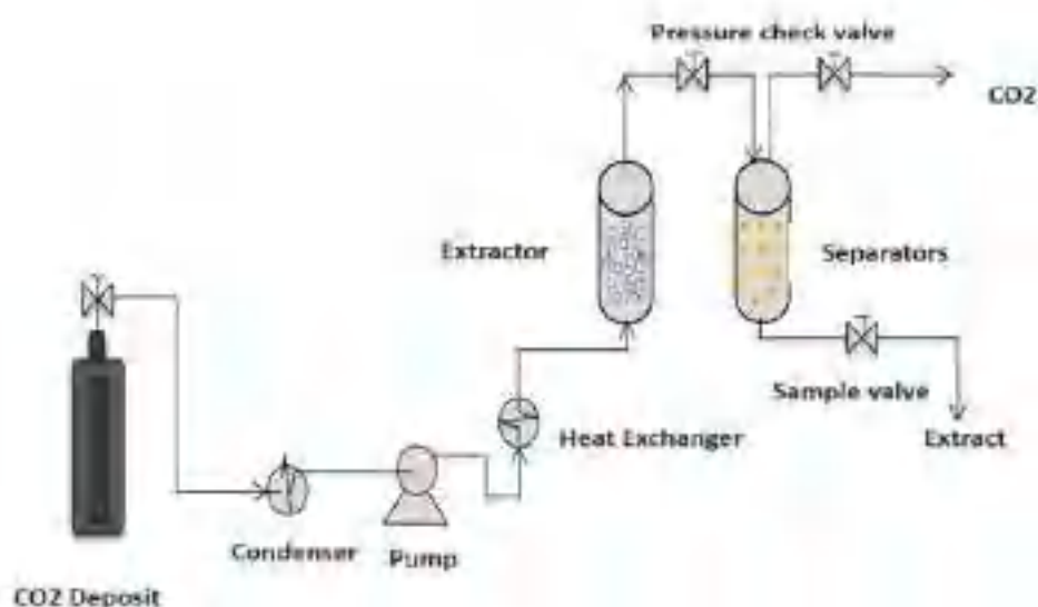
Figure 2. Scheme of CO 2 extractor
