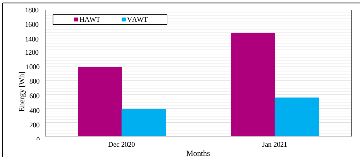
Figure 18. Total energy generated by HAWT and VAWT systems in December 2020 and January 2021
