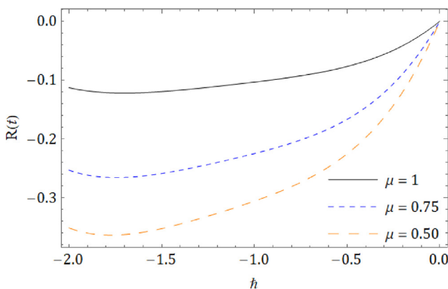
Fig. 4 \hbar -curves drawn for (i) S(t) , (ii) I(t) , (iii) R(t) with n = 1 and t = 0.01 for Case I at different \mu using Table 1.
