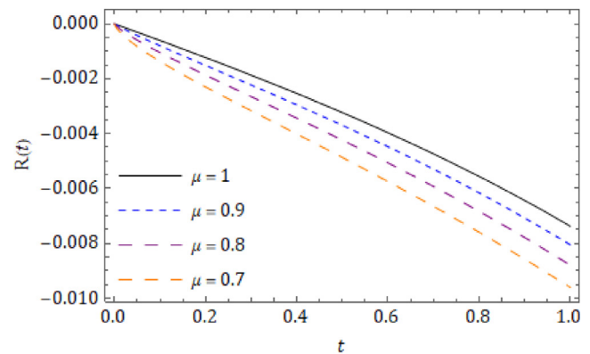
Fig. 5 Nature of q -HATM solution with t for (i) S(t) , (ii) I(t) , (iii) R(t) at \hbar = -1, n = 1 and using Table 1 for the Case II with diverse \mu .
