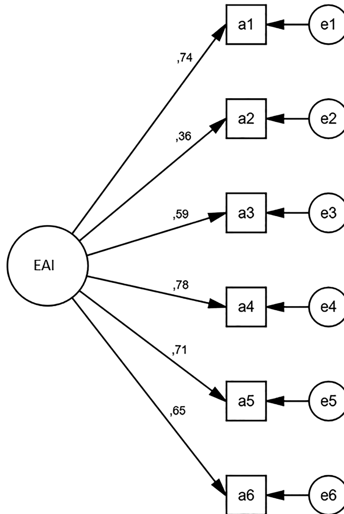
Figure 2. Confirmatory Factor Analysis Diagram for the Turkish Exercise Addiction Inventory. EAI: Exercise Addiction Inventory.
