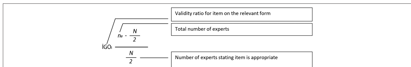
Figure 1. Formula 1-Lawshe Content Validity Formula.
