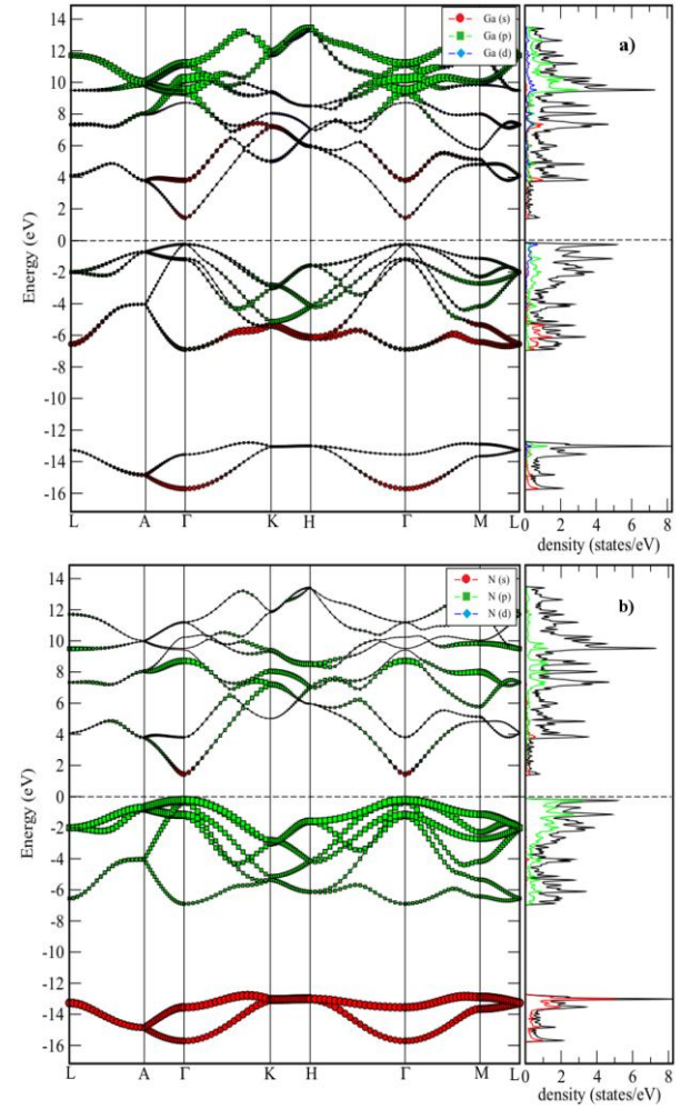
Figure 3. The calculated total energy bands and corresponding total a) Ga and b) N atoms partial DOS (pDOS) of GaN in the wurtzite (B4) phase. The line on the zero point represents Fermi level.
