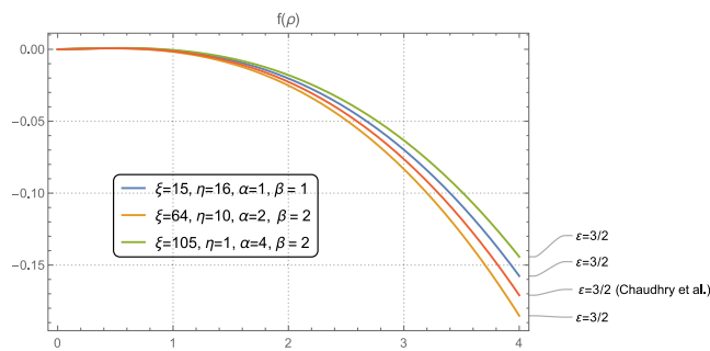
Fig. 1. The behavior of approximate solutions f(\rho) of Example 1 and Corollary 3.1 for \varepsilon = 3/2 , where p = q = 1 , x = y = 4 , 0 < \rho < 4 and generalized M-series and exponential series indexes n = 0, 1 .
