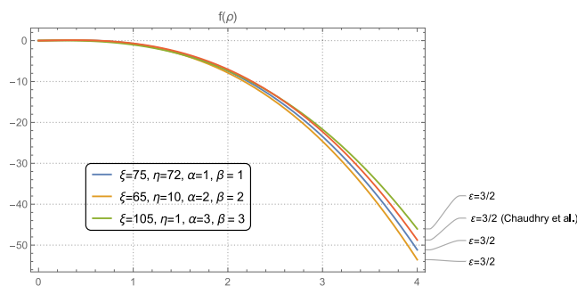
Fig. 2. The behavior of approximate solutions f(\rho) of Example 2 and Corollary 3.2 for \varepsilon = 3/2 , where p = q = 1 , \chi_1 = \chi_2 = 2 , \chi_3 = 4 , z = 1/2 , 0 < \rho < 4 and generalized M-series and exponential series indexes n = 0, 1 and modified Gauss hypergeometric series and generalized Gauss hypergeometric series indexes k = 0, 1 .
