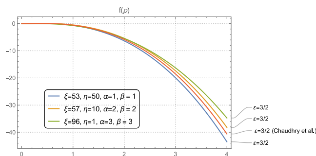
Fig. 3. The behavior of approximate solutions f(\rho) of Example 3 and Corollary 3.3 for \varepsilon = 3/2 , where p = q = 1 , \chi_2 = 2 , \chi_3 = 4 , z = 1/2 , 0 < \rho < 4 and generalized M-series and exponential series indexes n = 0, 1 , modified confluent hypergeometric series and generalized confluent hypergeometric series indexes k = 0, 1 .
