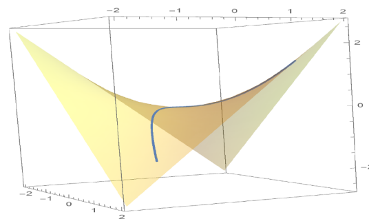
Fig. 1. For d_1 = 1 , d_2 = 2 , the spacelike helix \gamma lies on y = \frac{2}{3}xz .
