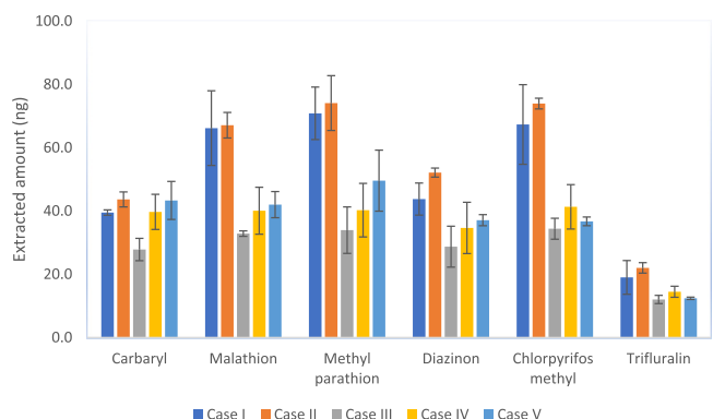
Fig. 5. Effect of sample centrifugation and filtration on the extraction of pesticides with TFME samplers ( n = 3 ). Extraction conditions: 40.0 mL sample volume (diluted apple juice (50:50)), 250.0 ng mL -1 analyte concentration, 1000 rpm agitation rate. Desorption conditions: 0.6 mL methanol, 60 min desorption at 1000 rpm agitation rate.
