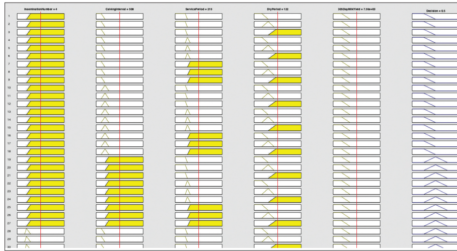
Fig 3. Rule viewer
