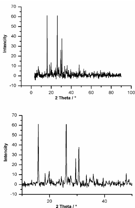
Graph 1. The XRD pattern of Davutoğlu clay
