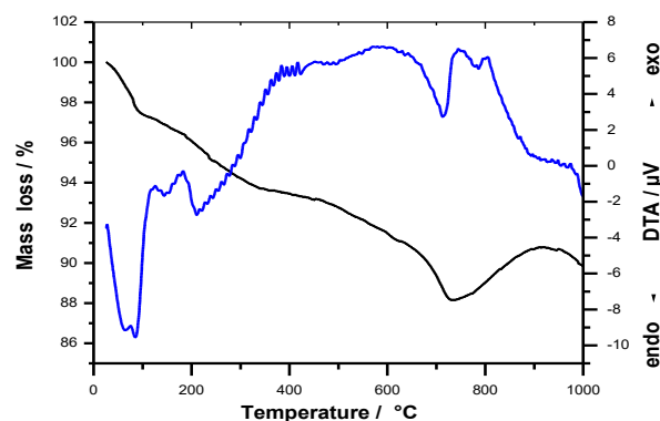
Graph 2. The TG-DTA curve of Davutoğlu clay. Black, TG; blue, DTA curves
