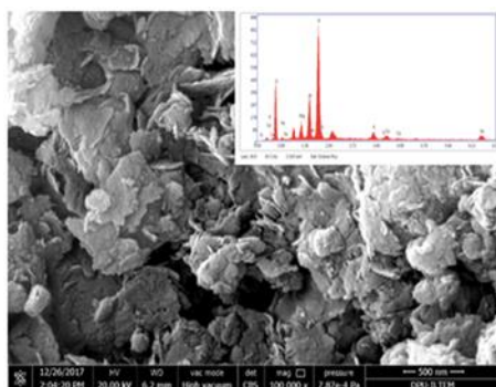
Picture 3. SEM analysis and EDX results of Davutoğlu clay XRF analysis shows large clay minerals in the clay material and some carbonates of the IIA group elements
