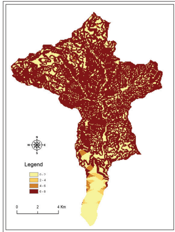
Fig.4. Slope Map
