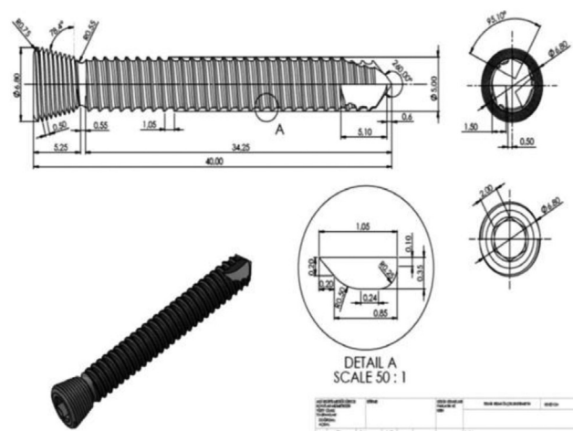
Fig. 2 – Cortical-bone screw-implant design [1].
